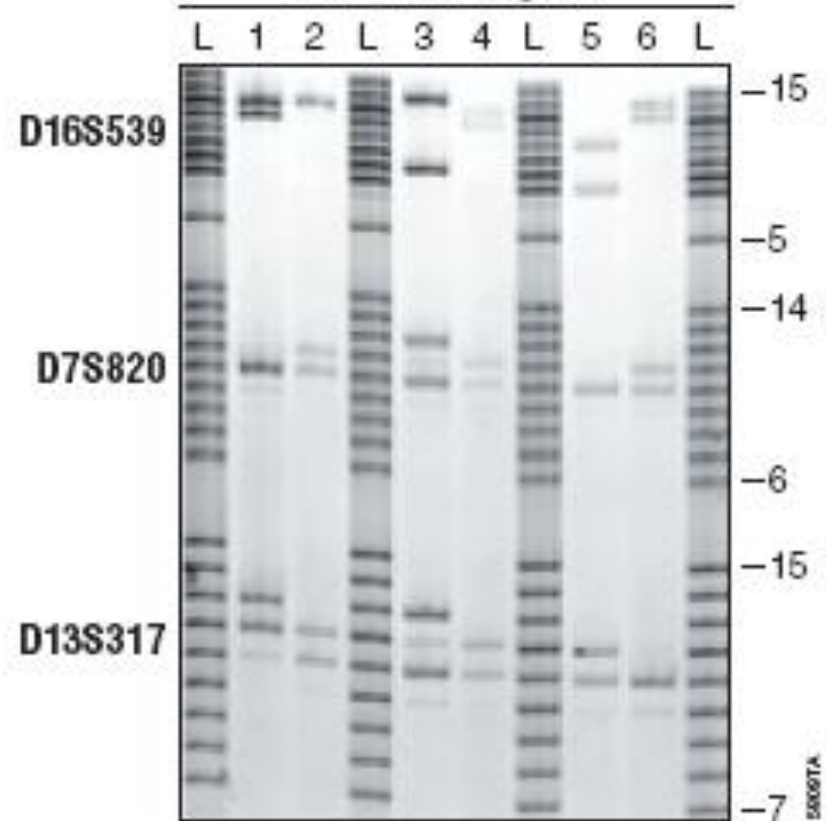
6% Denaturing Gel
